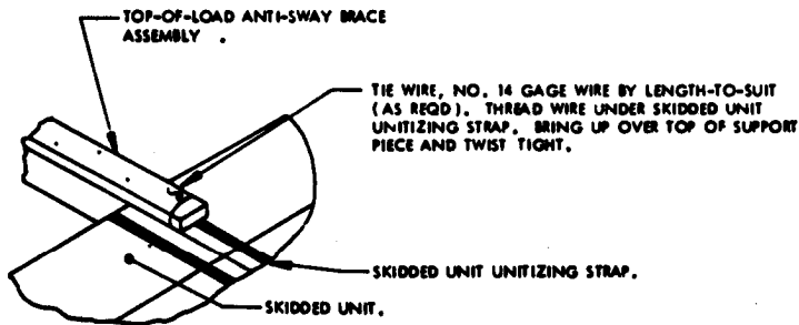
POSITIONING OF TOP-OF-LOAD ANTI-SWAY BRACE ASSEMBLY B
