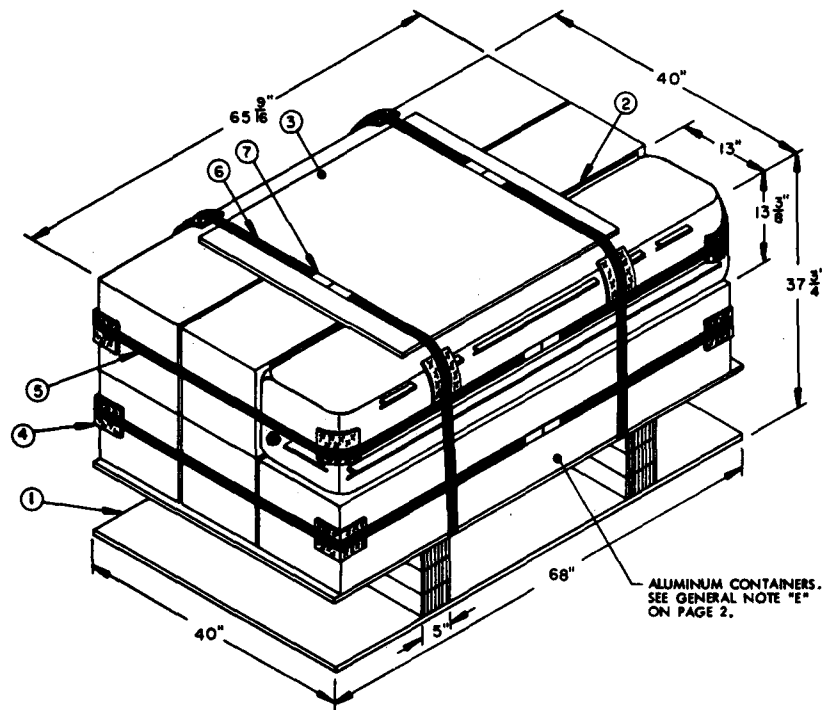
PALLETIZED UNIT
