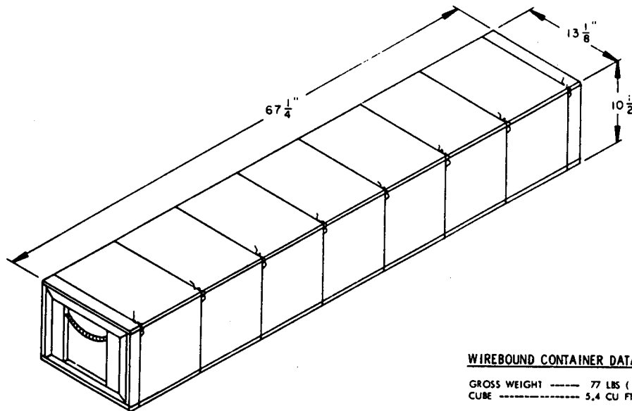
WIREBOUND CONTAINER
