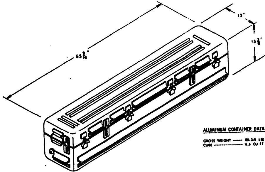
ALUMINUM CONTAINER
