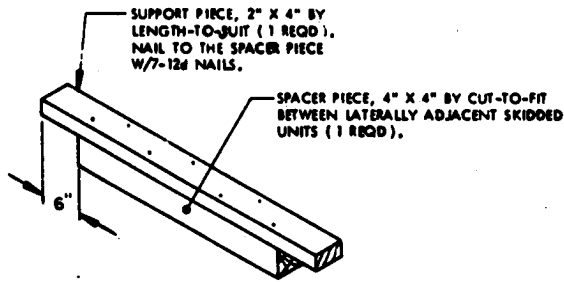
TOP-OF-LOAD ANTI-SWAY BRACE ASSEMBLY B
