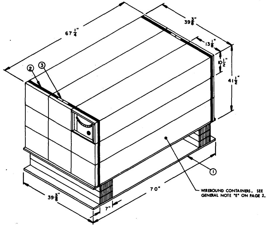
PALLETIZED UNIT
