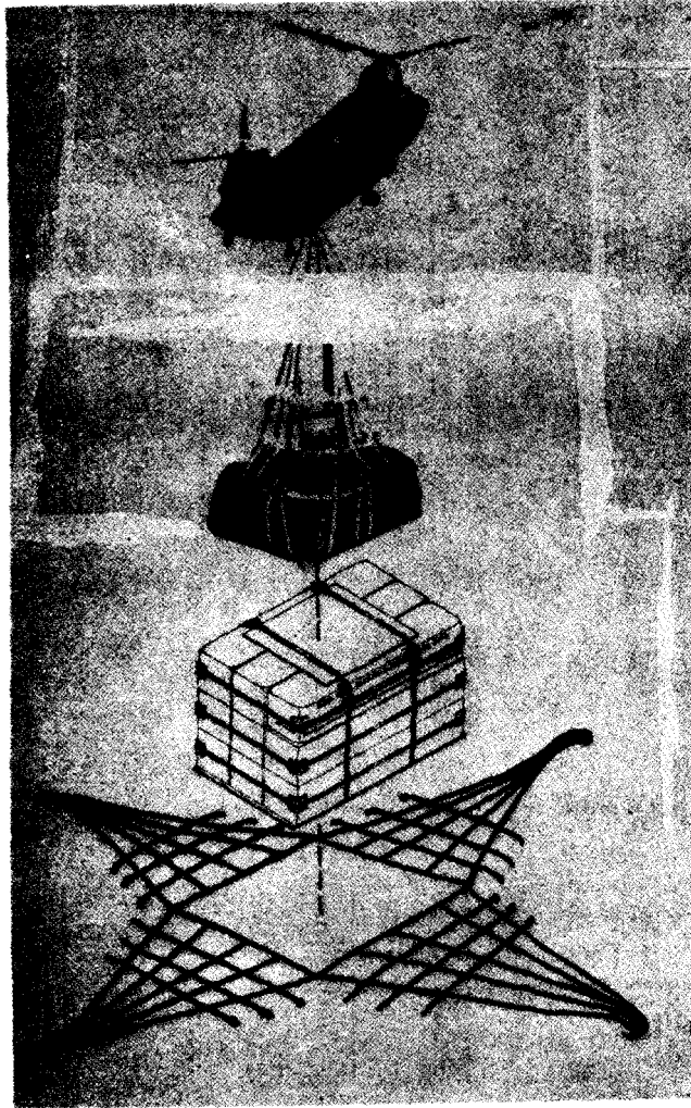
Figure 4-1. Assembly of nine STINGER weapon rounds or STINGER missile rounds in an A-22 aerial delivery bag for external transport by helicopter.
