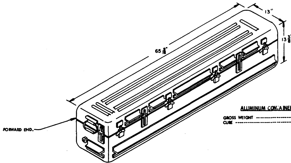
ALUMINUM CONTAINER
