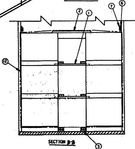
48 SKIDDED UNITS OF WIREBOUND CONTAINERS IN A 50'-6" LONG BY 9'-2" WIDE CONVENTIONAL BOX CAR
