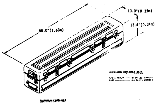
Figure 2-2. STINGER weapon round in shipping and storage container.
