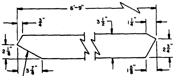
DIAGONAL BRACE D
