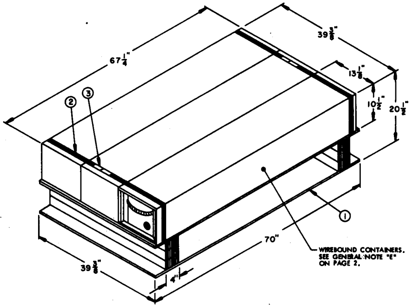
PALLETIZED UNIT
