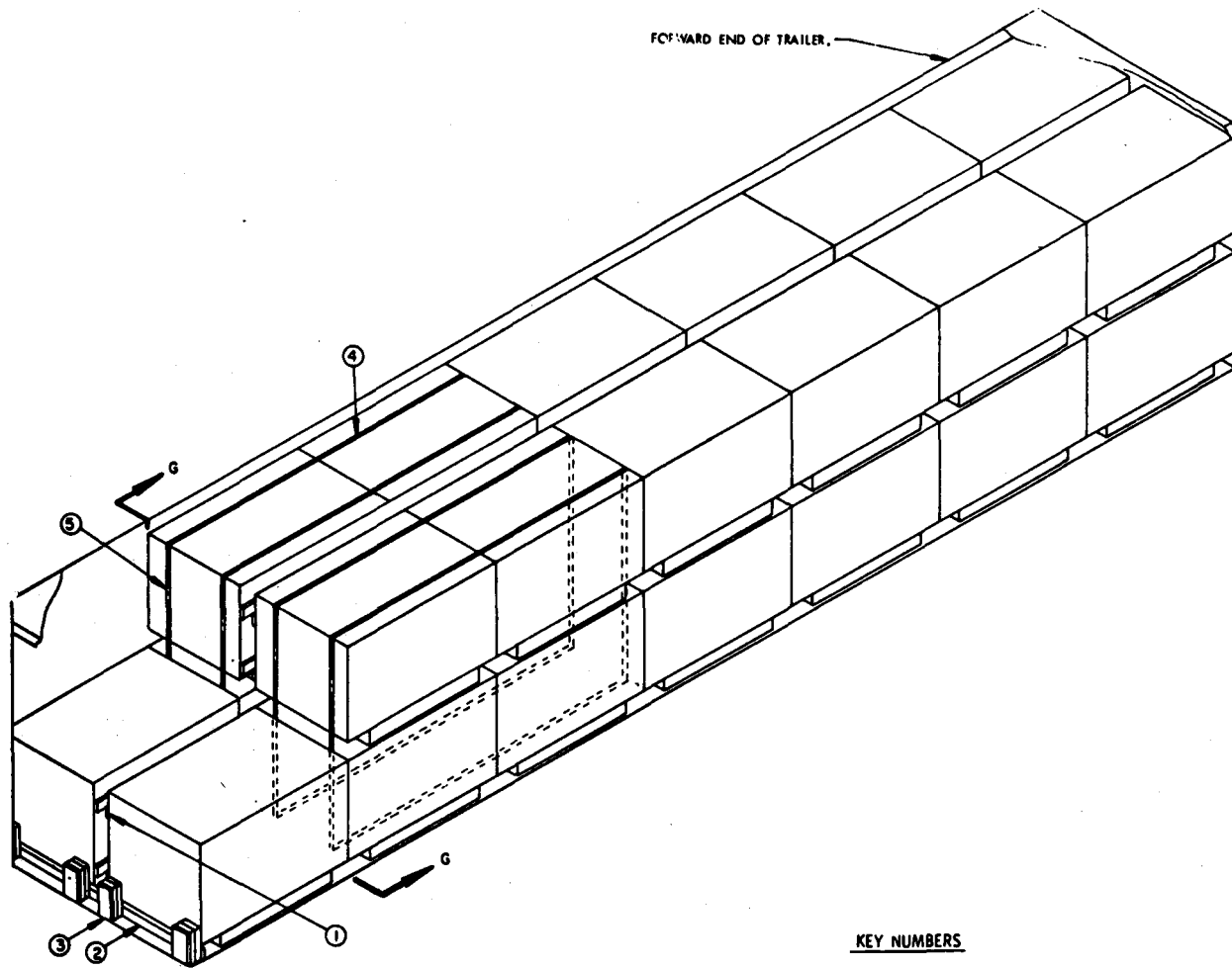
ISOMETRIC VIEW
