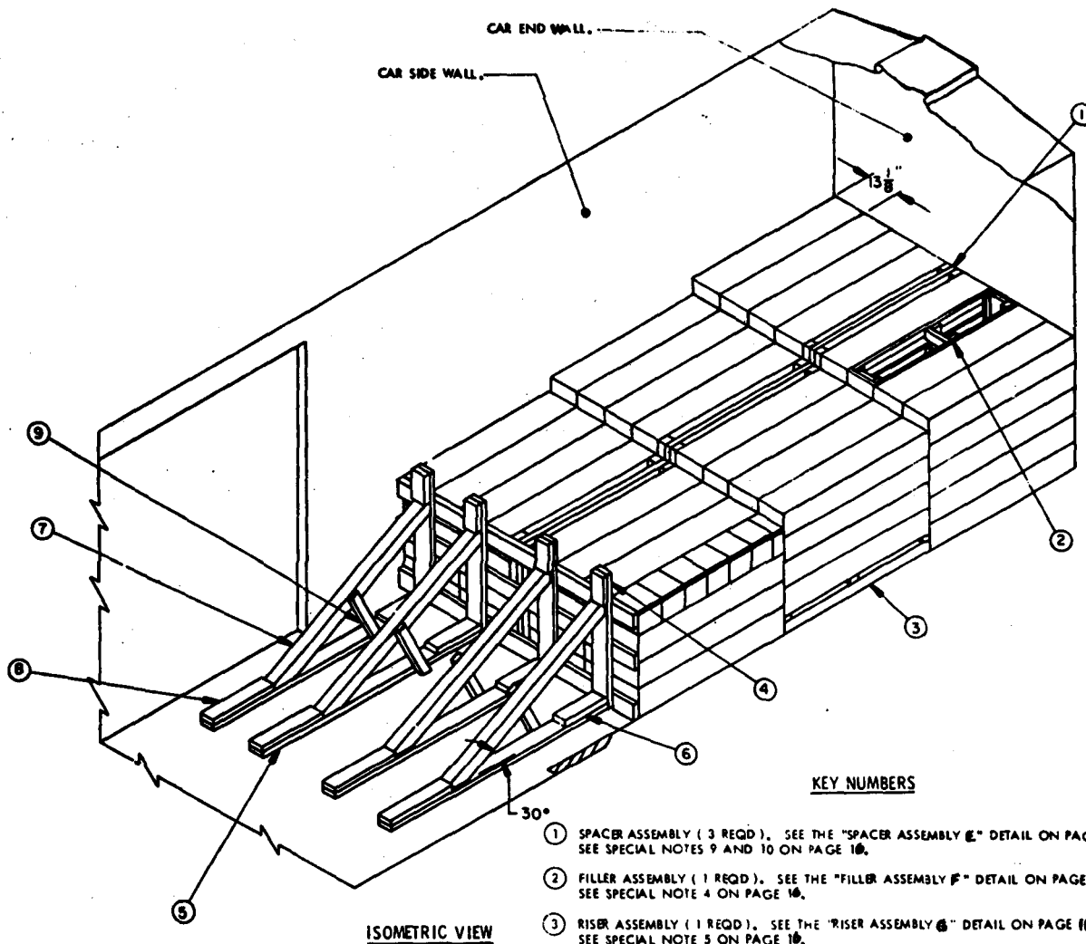
ISOMETRIC VIEW
