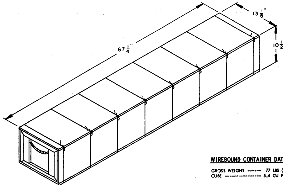
WIREBOUND CONTAINER
