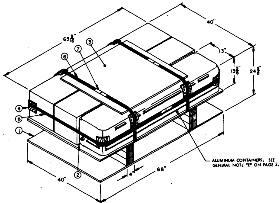
PALLETIZED UNIT
