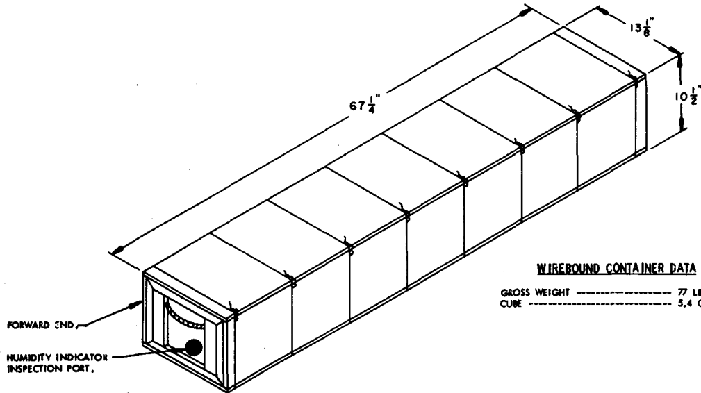
WIREBOUND CONTAINER
