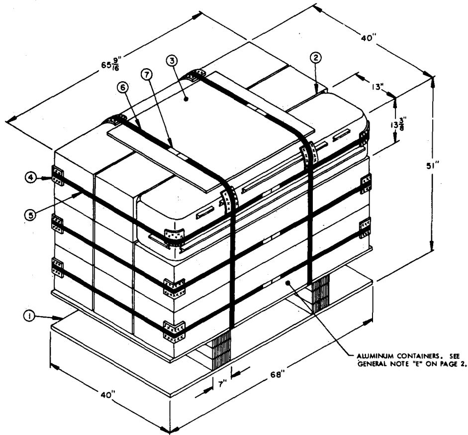
PALLETIZED UNIT
