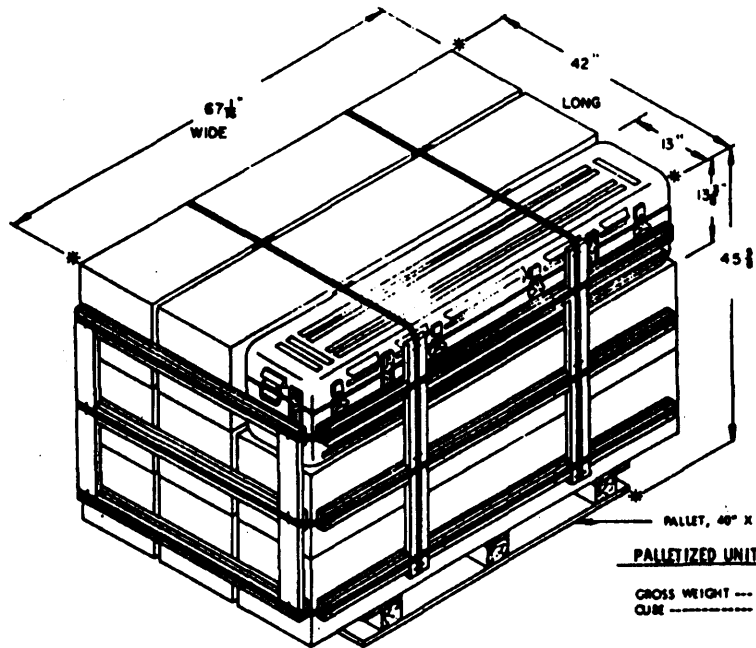
PALLETIZED UNIT OF NINE (9) GUIDED MISSILES. PACKED ONE (1) PER ALUMINUM CONTAINER.
