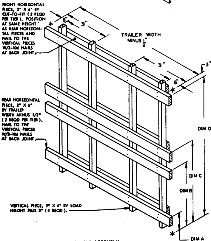
FORWARD BLOCKING ASSEMBLY SEE "NOTE ④", "NOTE ⑤", "NOTE ⑥" AND "CHART B" ON THIS PAGE.
