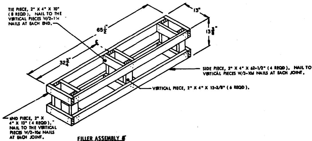
FILLER ASSEMBLY (E)
