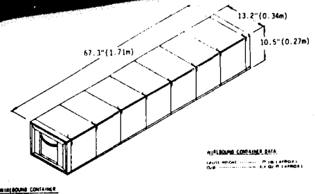
Figure 2-3. STINGER missile round in shipping and storage container.
