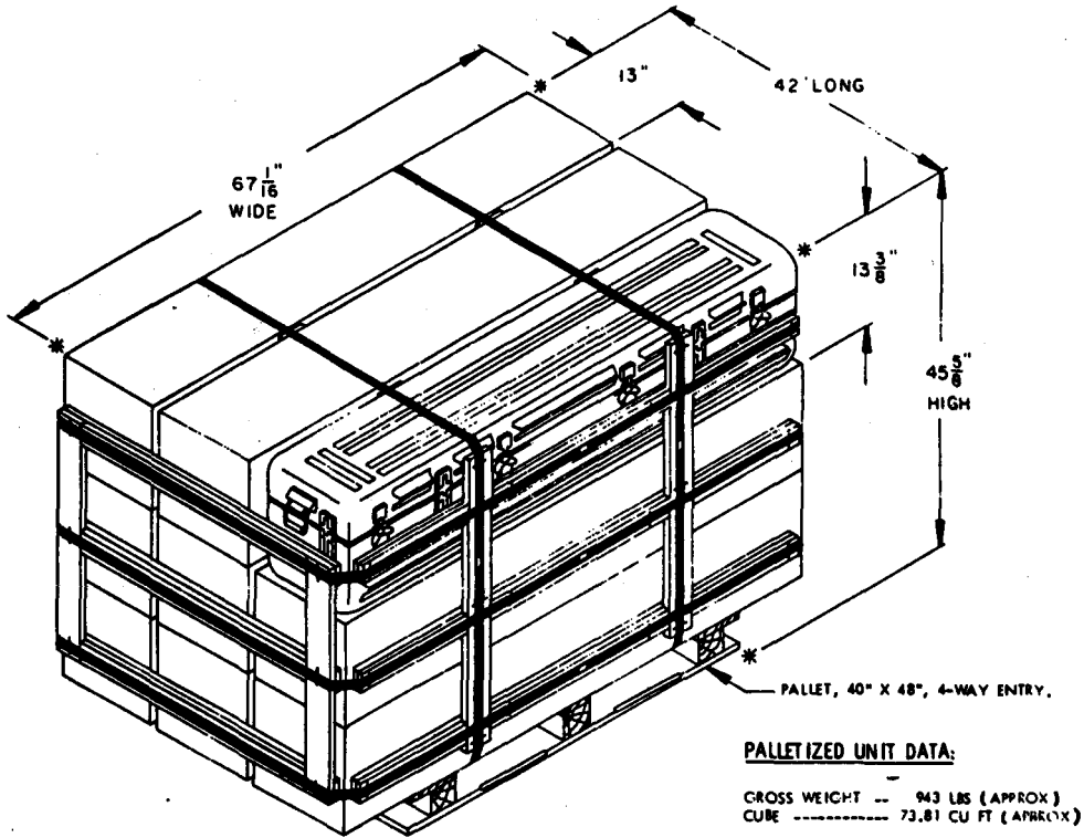
PALLETIZED UNIT OF NINE (9) GUIDED MISSILES, PACKED ONE (1) PER ALUMINUM CONTAINER.
